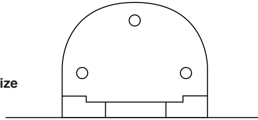
Side-Handle Hinge Layout
