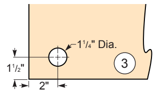
Power Cord Hole Location (Front View)
