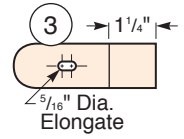
Swivel Arm (Front View)
