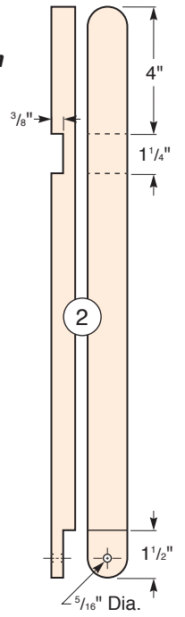
Swivel Arm (Front View)
