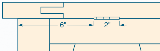
Hinge Locations (Back View)
