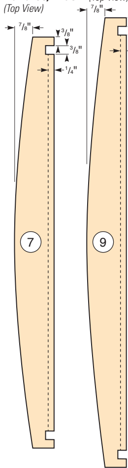
Top Tray Support Cross Bars (Top and Side Views)
