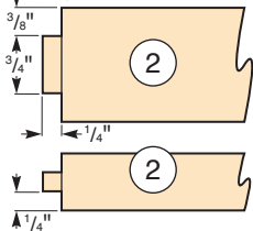
Top Tray Support Cross Bars (Top and Side Views)
