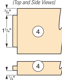
Wine Bottle Holder Mount (Top and Side Views)
