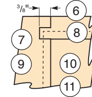
Tray Joinery Detail (Top View)
