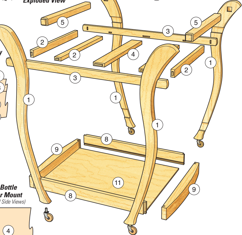
Exploded View
