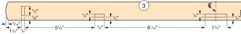
Top Tray Handles/Ends (Top View)
