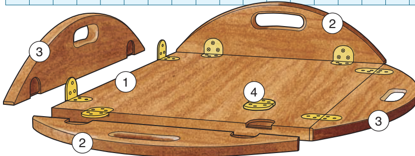
Exploded View
