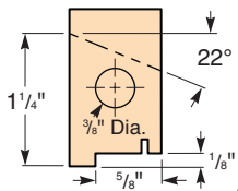
Upper Cross Braces (End View)
