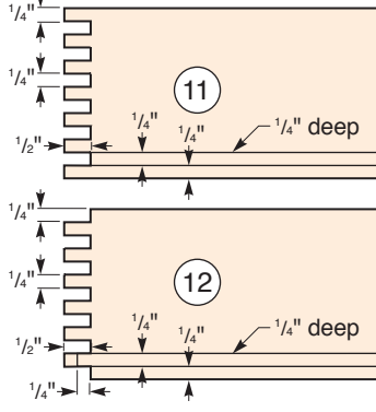
Lid Overhang (Side View)
