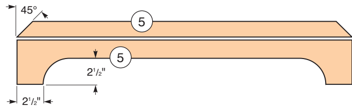
Base Front and Back (Front and Top Views)
