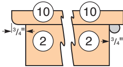
Lid Overhang (Side View)
