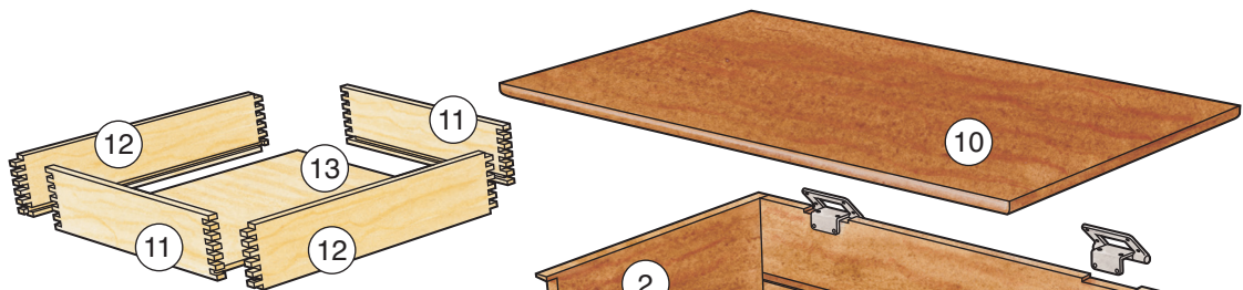
Tray Front, Back and Sides (Inside Views)
