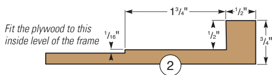
Octagon Segment (Section View)
