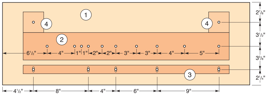
Dovetail Chiseling Jig (Top View)
