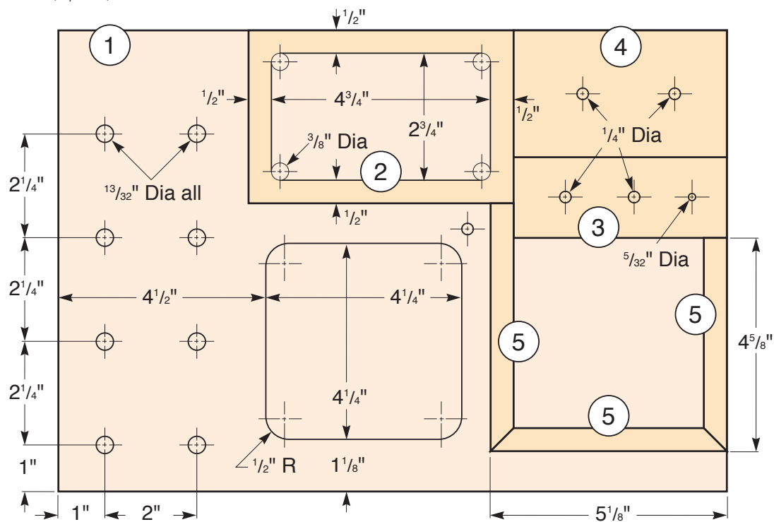
Drill Bit Organizer (Top View)
