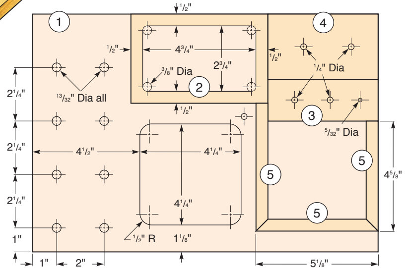
Drill Bit Organizer (Top View)
