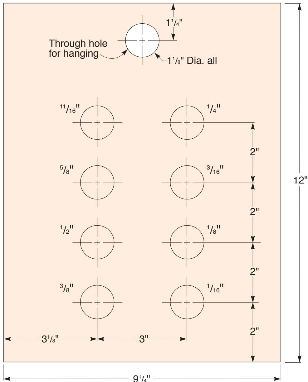
Depth Jig (Top View)
