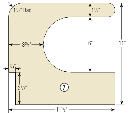
Drawer Front/Back
