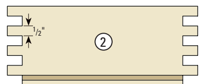
Carcass Front/Back
