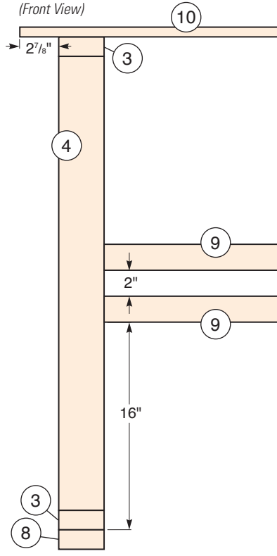
End of Table (Front View)
