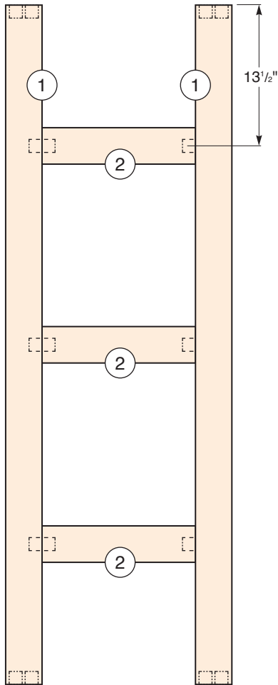
Upper Support Frame (Top View)
