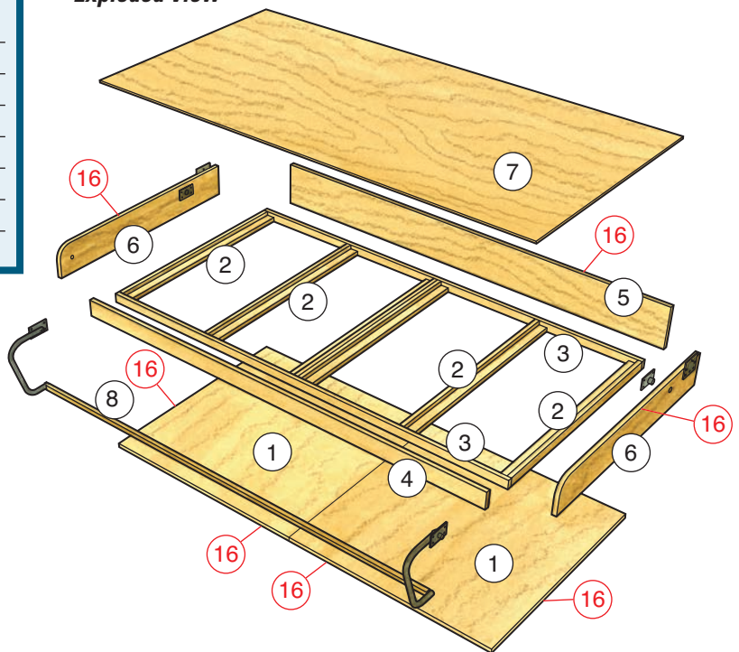
Bed Frame Exploded View
