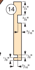
Drawer Side (Front View)
