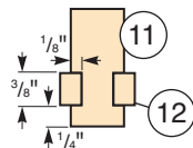
Drawer Runners (End View)
