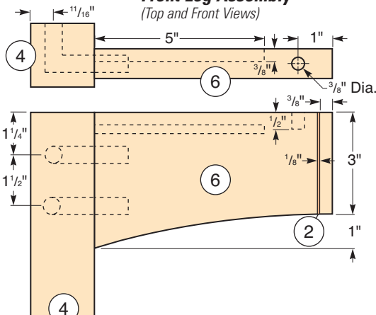
Front Leg Assembly (Top and Front Views)
