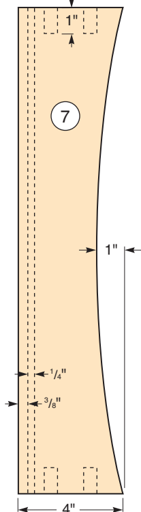
Side Apron (Front View)
