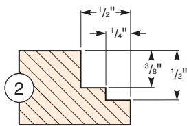
Mirror Rabbets (Section View)
