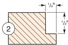
Photo Rabbet (Section View)
