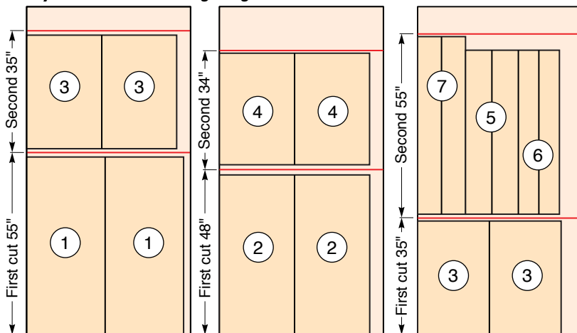
Plywood Sheets Cutting Diagrams
