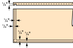
Drawer Joinery (Top and Inside Views)
