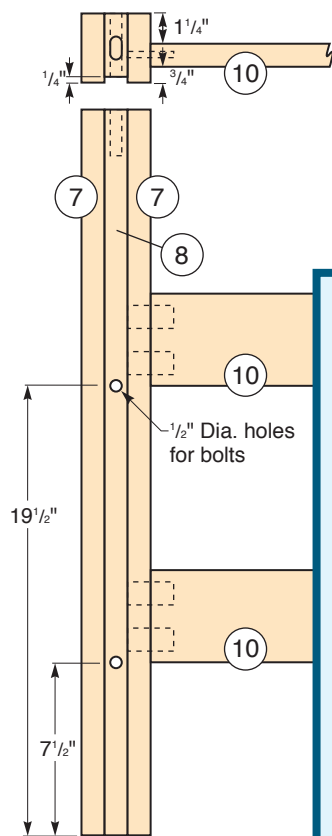
Leg and Rail Assembly (Top and End Views)
