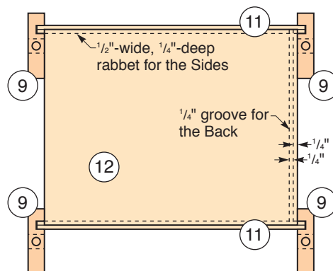
Drawer Housing and Rail Assembly (End View)
