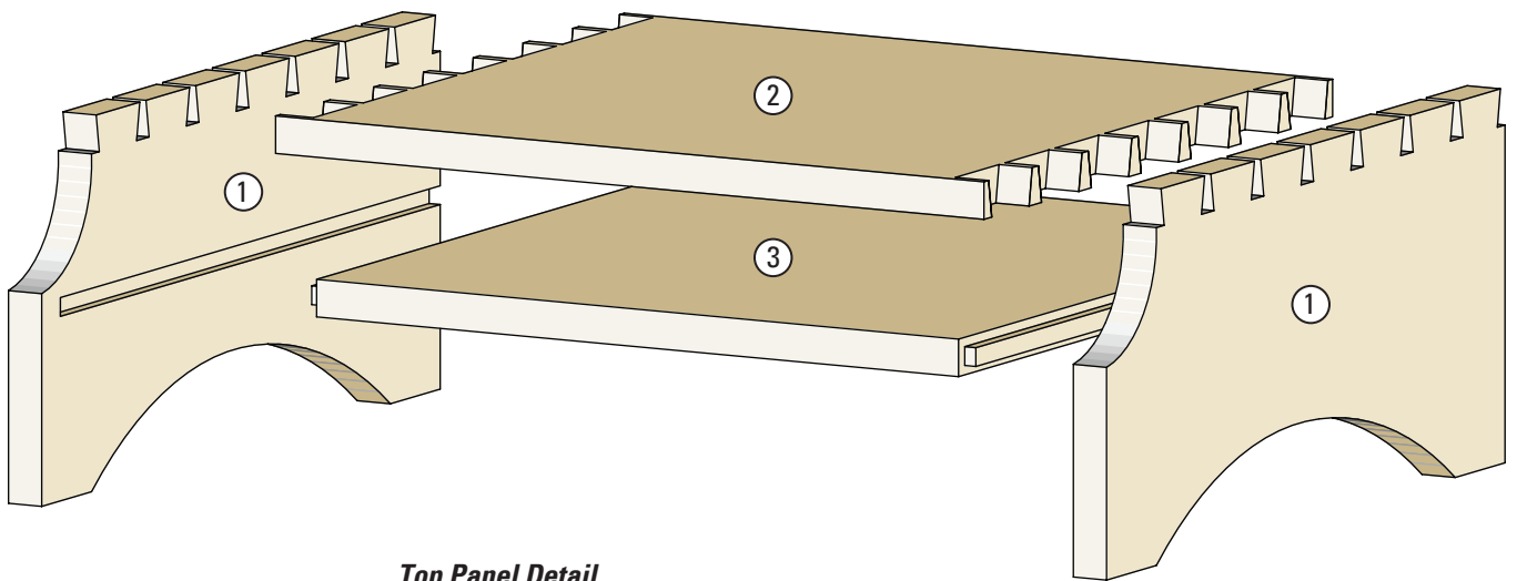
Top Panel Detail
