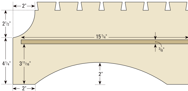
Side Panel Detail
