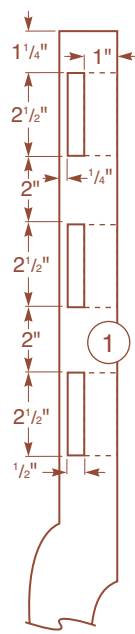
Left Rear Leg (Front View)
