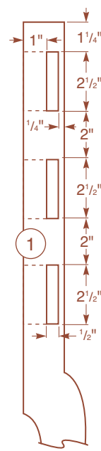
Left Rear Leg (Inside View)
