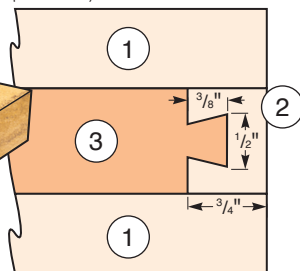
Dovetail (End View)
