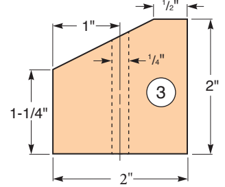
Hold-down Support (End View)
