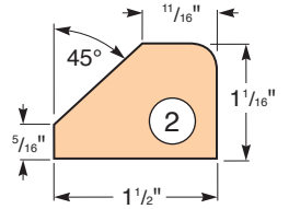
Hold-down Support (End View)
