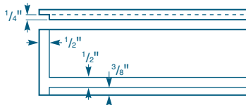
Drawer Sides (Top and Inside Views)
