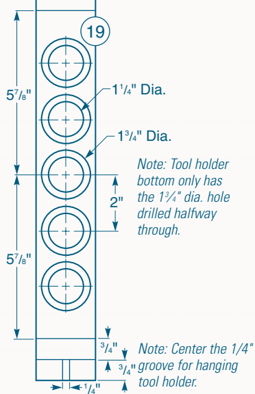
Tool Holder Top (Bottom View)
