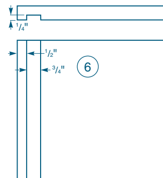
Side Panel (Inside and Top Views)
