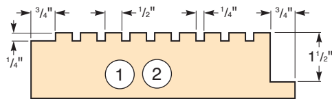
Middle and End Supports (Side View)
