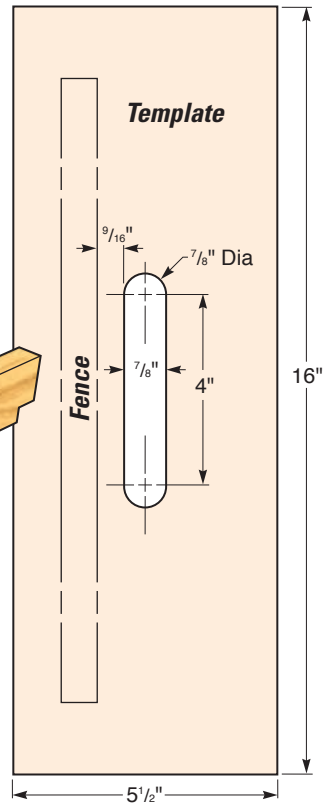
Routing Template (Top View)
