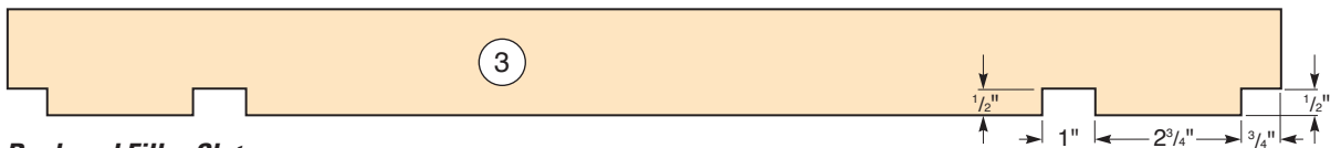
Back and Filler Slats (Front View)
