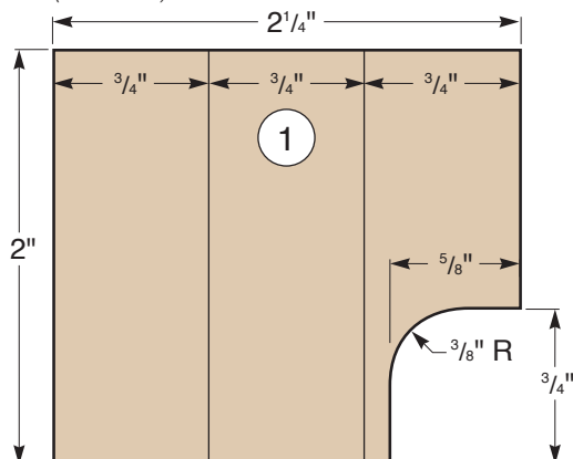
Cove Layout (End View)
