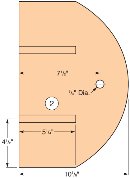
Bottom Shelf (Top View)
