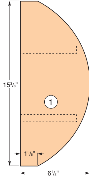
Bottle Holder (Front View)
