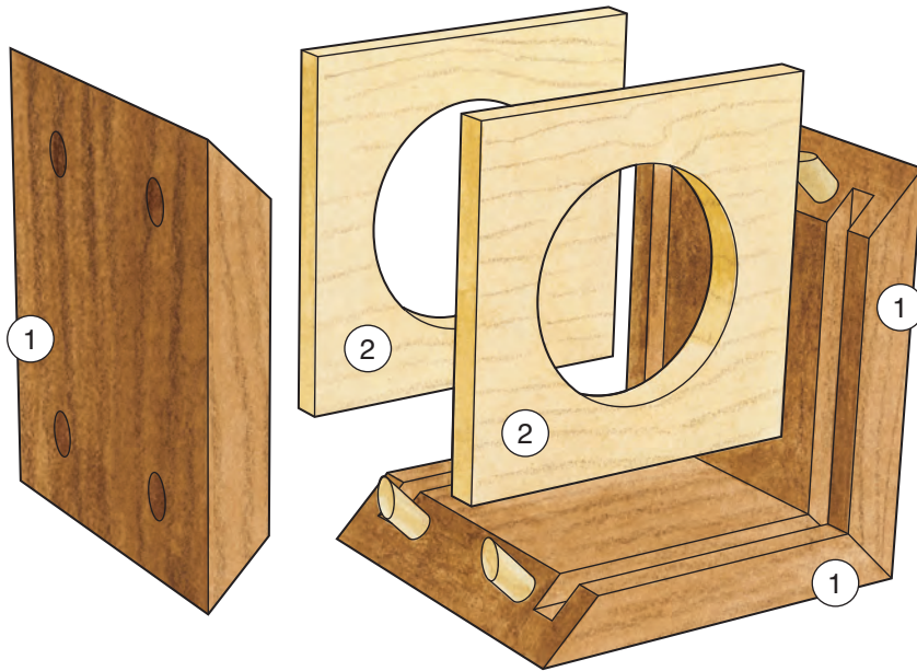
Exploded View
