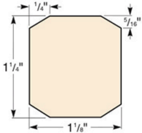
Shaft Blank Section View
